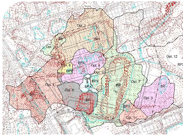
T:Rain Model
