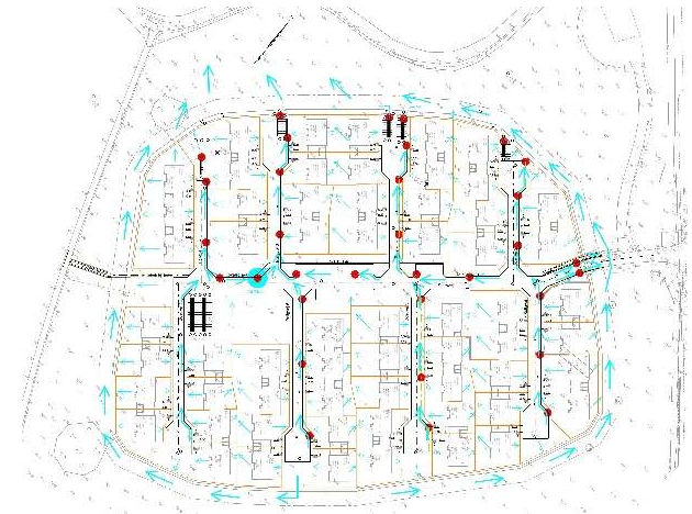
T:APi model
